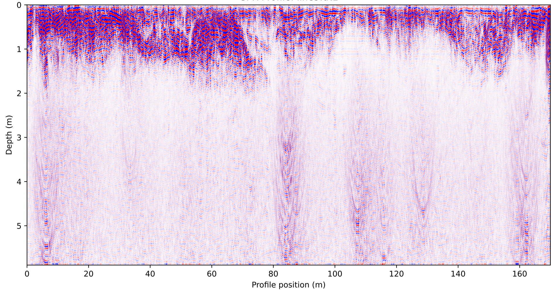
GPR Profile: line5.dt1
